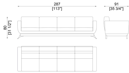
SC1010/4P Four-seat sofa Divano quattro posti
